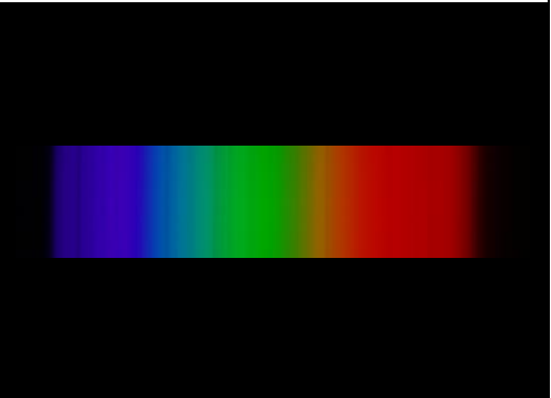
Spectre du Soleil
